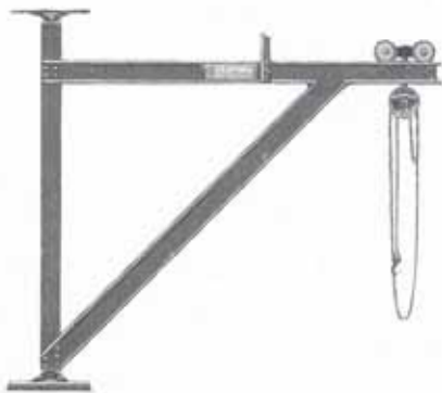
Type 2—Underbraced Jib Crane \frac{1}{2} to 2-ton capacity
