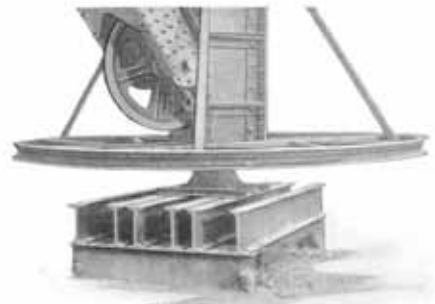
Base of derrick showing 7' 6" Bull Wheel
