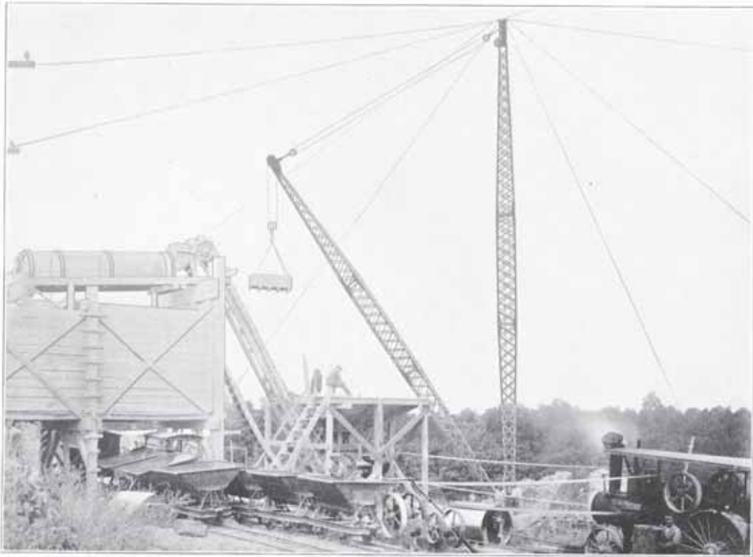
10-ton Bedford Steel Derrick, 80' 0" Boom, 90' 0" Mast
