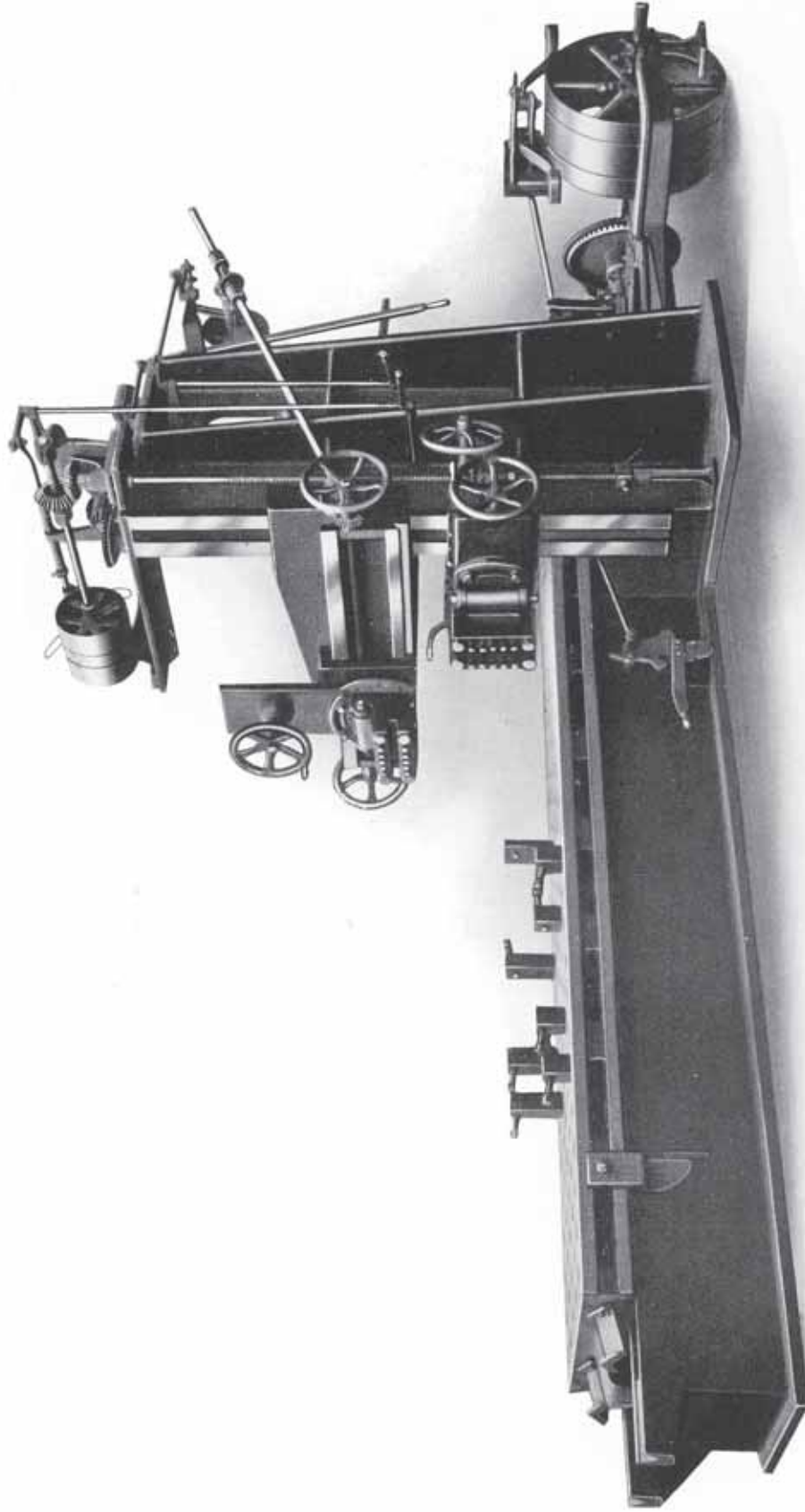
Standard 42" x 42" x 12' 0" Openside Worm-driven Planer. Latest Pattern.
