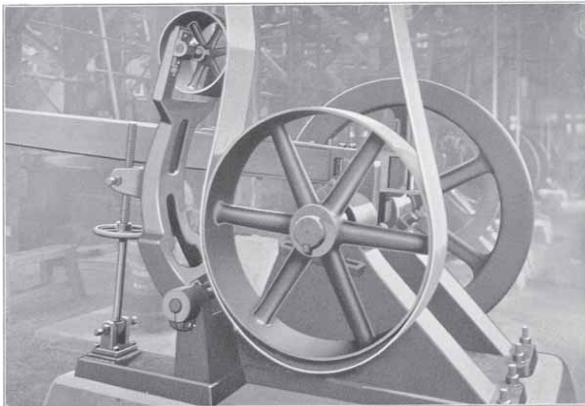
One Piece Box Type Hurst Frame, showing Adjustable Belt Tightener
