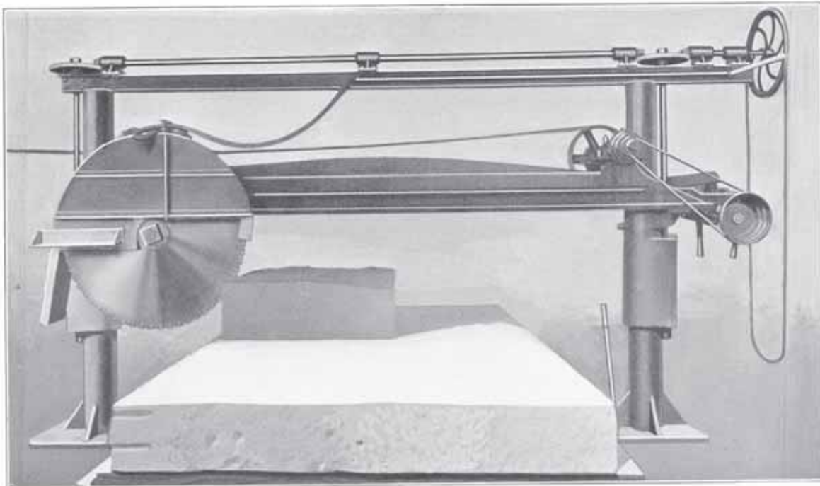
36" Diameter 8' 0" Rip, Belt Driven Diamond Saw. Single Truck
